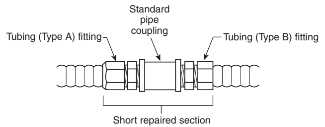
EXHIBIT S2.1 Repair Method for Damaged CSST Tubing Run. (Courtesy of Foster-Miller, Inc.)
